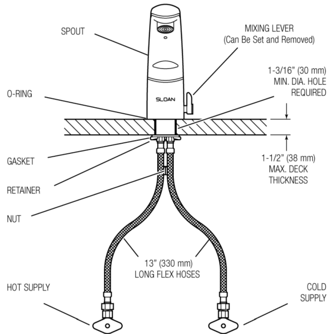
EF-150-ISM, EF-150-ISM-IQ AND EF-150-ISM-DPU-IQ Faucets with Hot and Cold Water Supply
