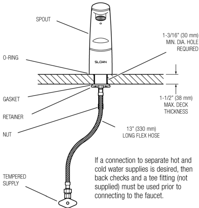
EF-150 AND EF-150-IQ Faucets with Single Line Water Supply
