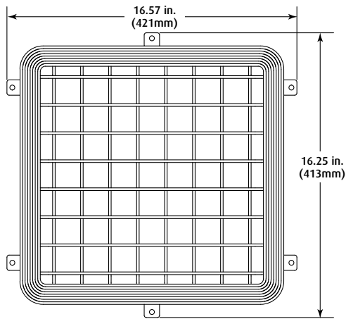
EXTERNAL DIMENSIONS
