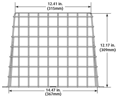
INTERNAL DIMENSIONS
