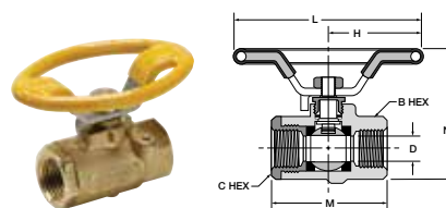
Oval Handle, Female Pipe Ends, Panel Mount XV502P-X-21
