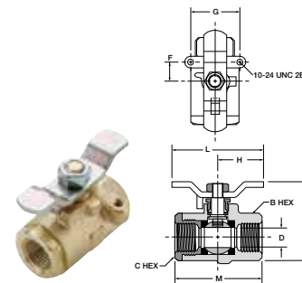
Tee Handle, Female Pipe Ends, Panel Mount XV502P-X-04
