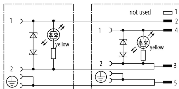
Valve plug 2
