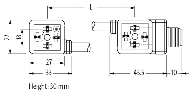
Valve plug 2
