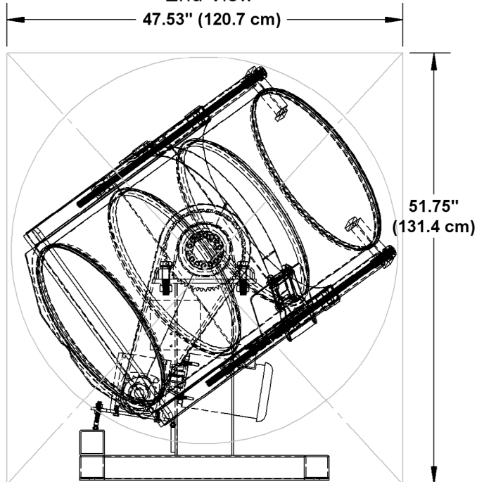
End View
