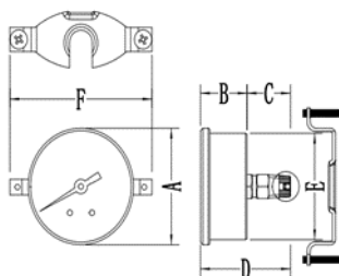
Back Mount with U-Clamp
