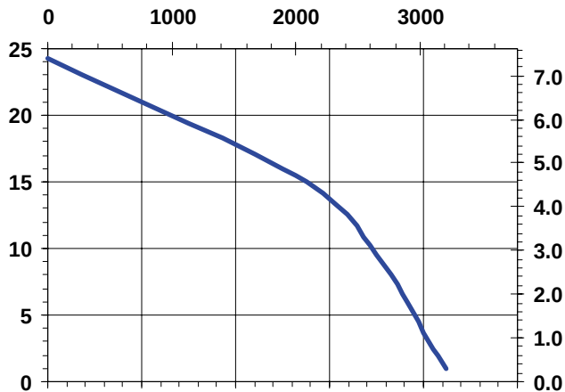
FLOW - LITERS/HOUR
