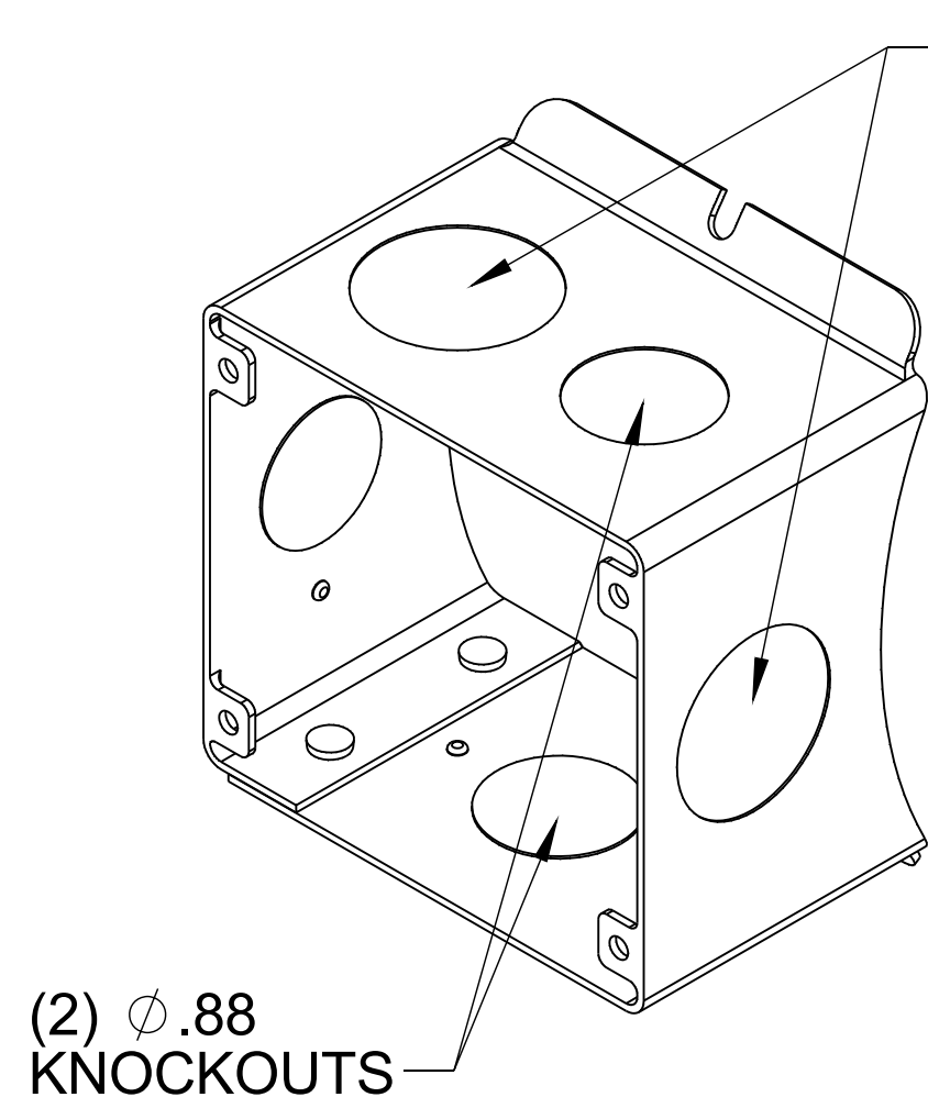
KNOCKOUT LOCATION DETAIL VIEW
