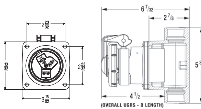
Breach Cap model shown. Flip Cap model dimensions are similar
