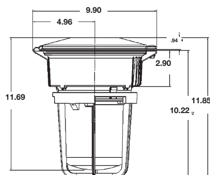
MBL Pendant, Refractor, Guard
