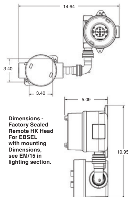
Dimensions - EBS with EL-EXIT &amp; HK Heads
