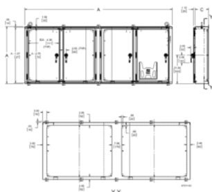
Four-Door Enclosure
