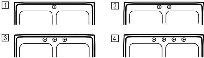
1-1/2" (38mm) Diameter Faucet Holes on 4" (102mm) Centers
