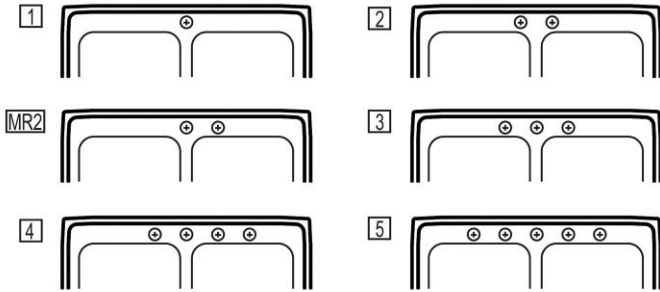
1-1/2" (38mm) Diameter Faucet Holes on 4" (102mm) Centers
