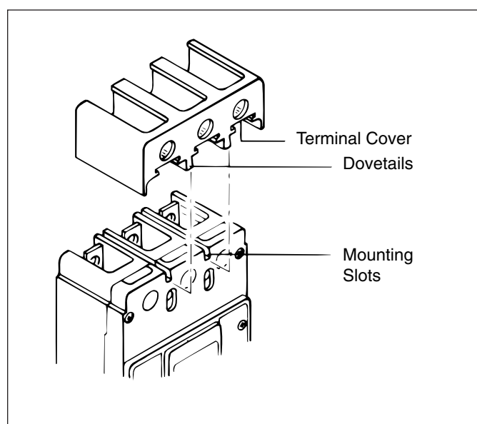
Figure 2-3 Terminal Cover Installation
