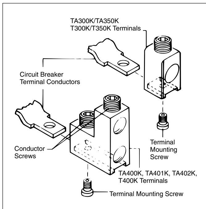
Figure 2-4 Terminal Installation
