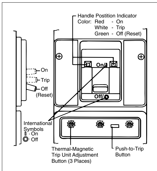
Figure 4-1 Circuit Breaker Manual Controls
