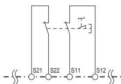
Fct.: E-stop (1), with cross fault detection SIL 3, PL e, Cat. 4
