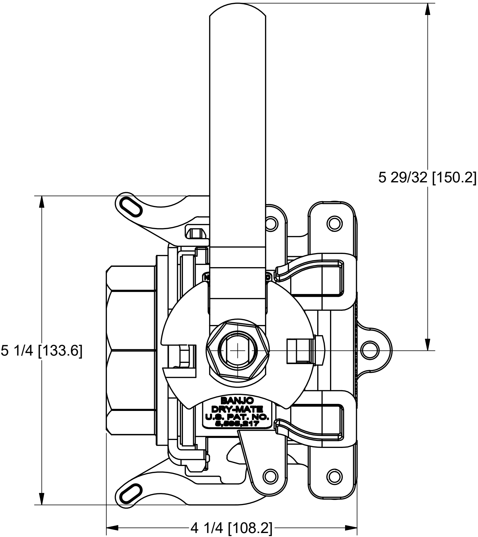
HANDLE IN CLOSED POSITION
