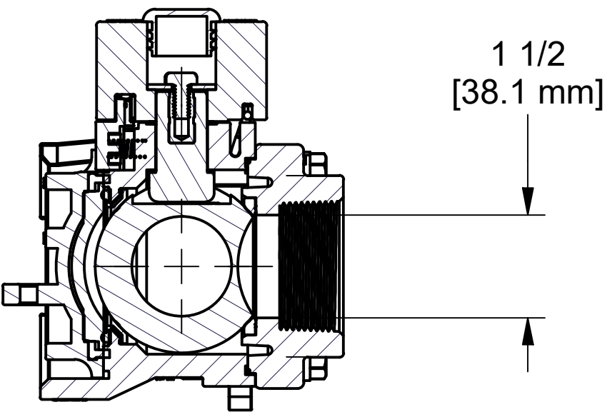
SECTION B-B SCALE 1 / 2
