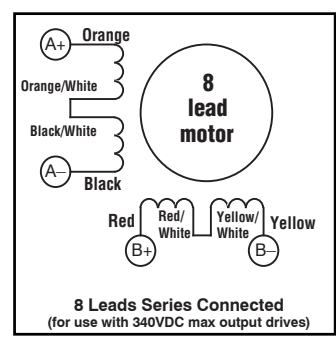
STP-MTRAC-34075(x), 34115(x) Motor Wiring
