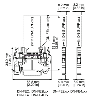
DN-FE2, DN-FE2Lxx, DN-FE4, DN-FE4Lxx DN-DIS-xxx dimensions are the same as DN-FExxx dimensions.
