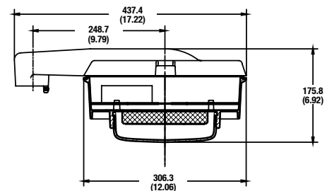
Stanchion Mount
