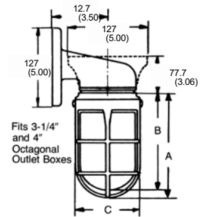
Types OBV and OBVW
