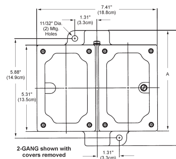
2-Gang Front View
