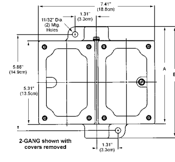
2-Gang Front View
