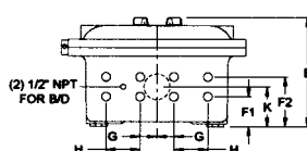
Panel D – End View
