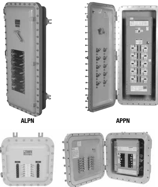
AGPN shown with MB and INV options
