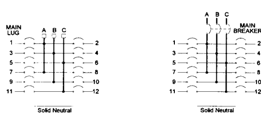
3-Phase, 4-Wire Systems
