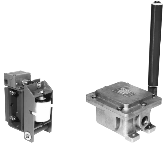
AFA1, AFA2, AFAX1, AFAX2 Large Roller Style
