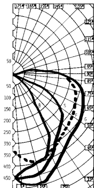
A-51 Incandescent Fixture with 30° Reflector
